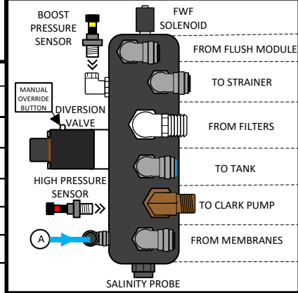
Detail View 1: Plumbing Manifold
