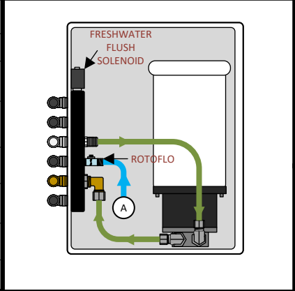
Detail View 2: Feed Pump Module Internals
