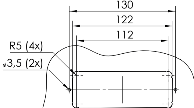
Mounting dimensions remote panel
