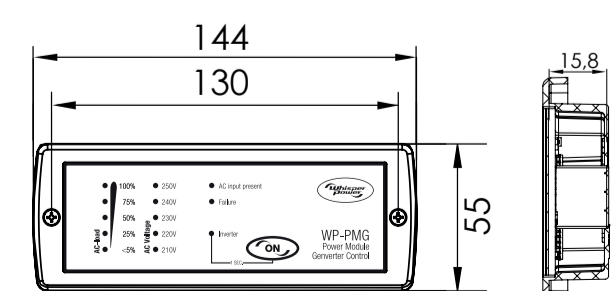
Front and side view remote panel
