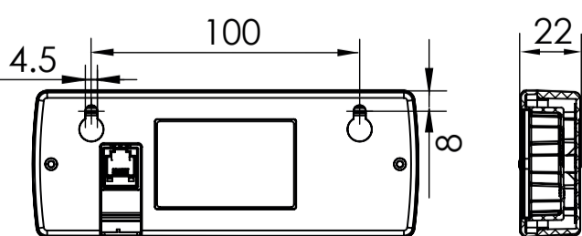
Rear and side view remote panel
