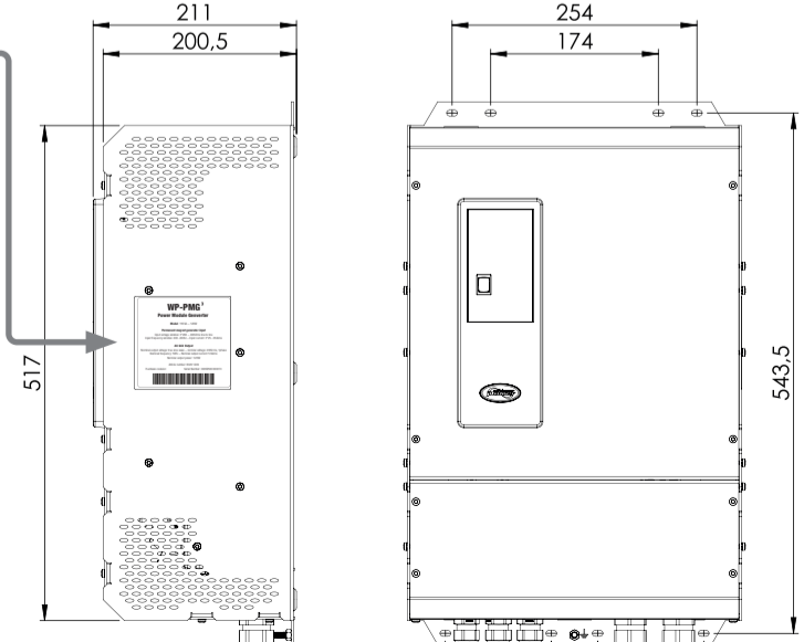
Front and side view WP-PMG
